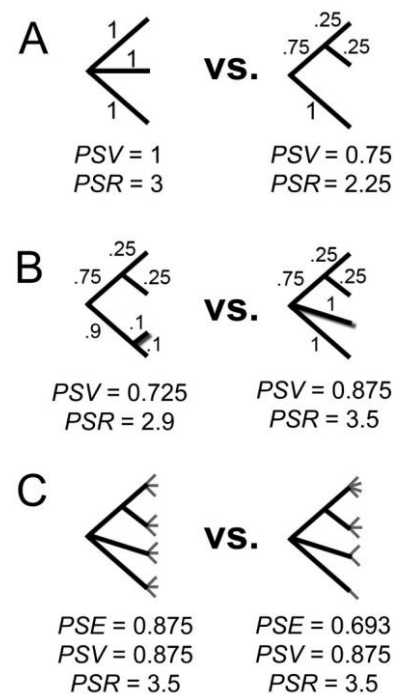
Figure 1: Phylogenies with values for the metrics of phylogenetic species variability (PSV), phylogenetic species richness (PSR), and phylogenetic species evenness (PSE). A, PSV and PSR are at their maxima (1 and species richness, respectively) when a community phylogeny is a star. Because two species of the right-hand phylogeny are related, PSV and PSR values are less than the values of the left-hand phylogeny. B, When a species is added to a community, the resulting values of PSV and PSR are dependent on the species branch length and where on the phylogeny the species is added. Relative to the right-hand phylogeny of A, PSV decreased in the left-hand phylogeny of B, while PSV increased in the right-hand phylogeny of B. C, Our metric PSE essentially grafts each individual of a community onto the tip of the phylogeny of its species with branch lengths of 0. For the left-hand phylogeny, PSE is equal to PSV because all species abundances are equal. When abundances are uneven, PSE is generally less than PSV, as in the right-hand phylogeny. When species are phylogenetically even, as in the left-hand phylogeny of A, and have even abundances, PSE = 1 .
