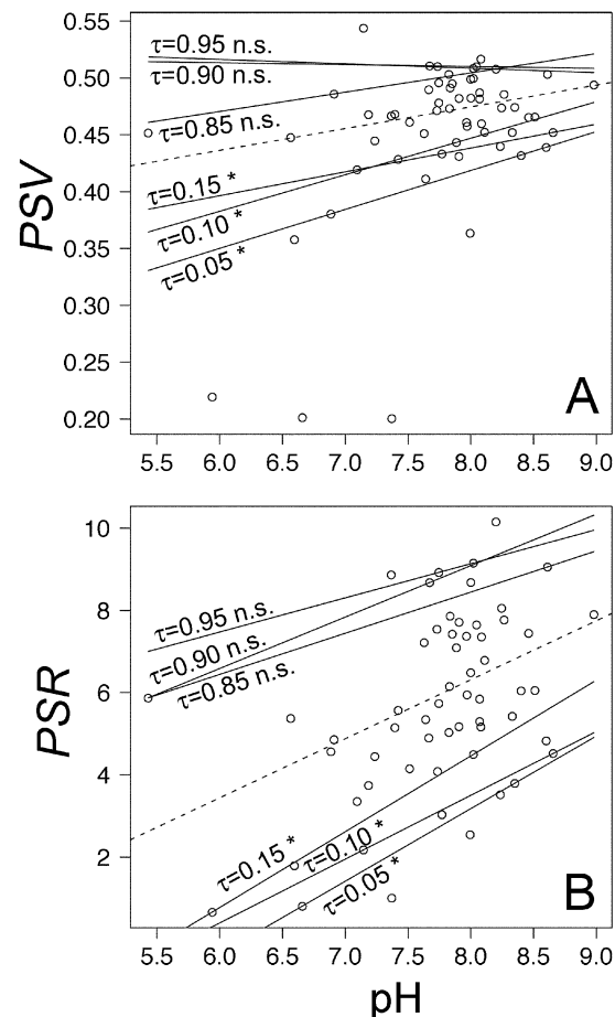
Figure 4: Quantile regressions ( solid lines ) of phylogenetic species variability (PSV; A ) and phylogenetic species richness (PSR; B ) of lake fish communities show pH to be significant only at the lower ends of the metrics' distributions. Regressions are weighted by the inverse of the expected variance of PSV and PSR. Asterisks denote a quantile regression pH coefficient to be significant (see "Methods"), while n.s. indicates no statistical difference from 0. Dashed lines are weighted least squares regressions.
