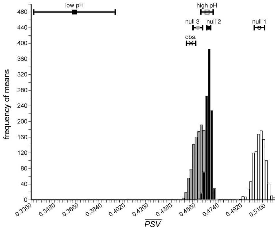
Figure 3: Observed and permuted mean phylogenetic species variability ( \overline{PSV} ) values for northern Wisconsin lake fish communities. Null distributions are produced from 1,000 permutations of the data set under null models 1 (white bars), 2 (black bars), and 3 (gray bars). Circles directly above histograms are the means of those distributions \pm 1 SE. The observed mean PSV value (cross) is indicated, with \pm 1 SE calculated by combining the variances of each community (eq. [3]). The fish communities are phylogenetically underdispersed according to nulls 1 and 2, but not null 3, because the observed mean is below the null 1 and 2 distributions but within the 0.005 and 0.995 quantiles of the null 3 distribution ( \alpha = 0.01 ). Squares are the mean PSV values of the subset analysis, \pm 1 SE (see “Methods” for standard error calculation). Low-pH lakes contain species with significantly less phylogenetic species variability than do high-pH lakes.
