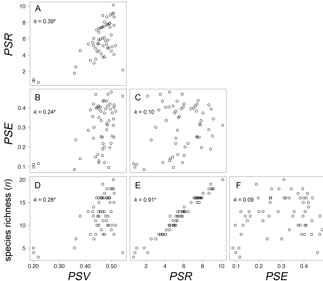
Figure 2: Fish community scatterplots of species richness ( n ), phylogenetic species variability (PSV), phylogenetic species richness (PSR), and phylogenetic species evenness (PSE). Asterisks indicate nonparametric Kendall rank correlations ( k ) that are significant at \alpha = 0.01 .
